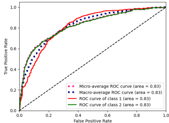
Figure 1 ROC analysis of LGB ML model.
