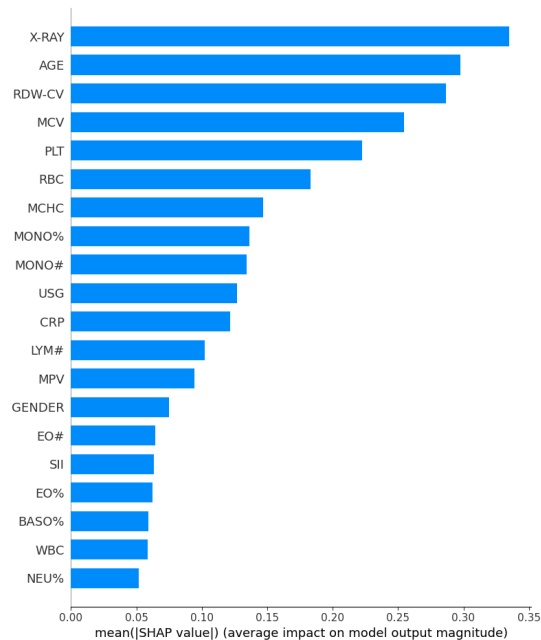
Figure 3. SHAP analysis for LGB ML model.
