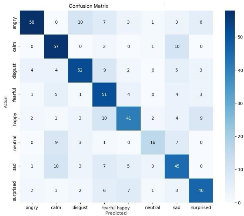
Figure 1: Confusion Matrix of the Test Set
