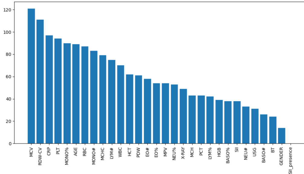
Figure 2. Feature importance analysis for LGB ML model.
